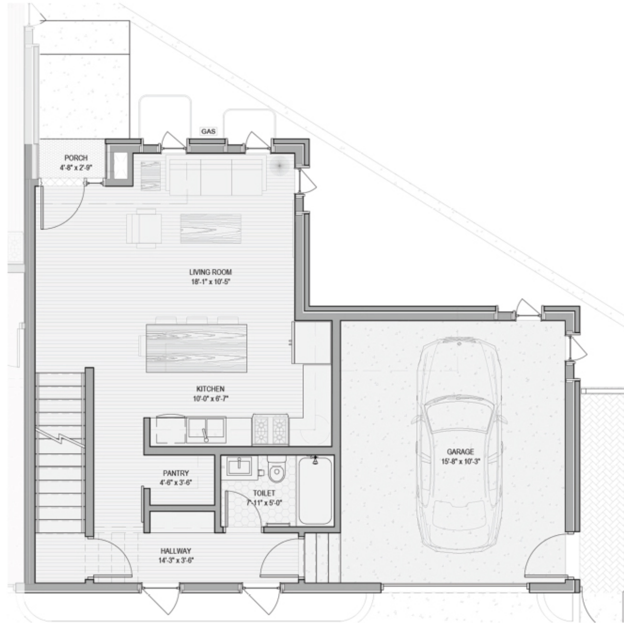
FIRST FLOOR
