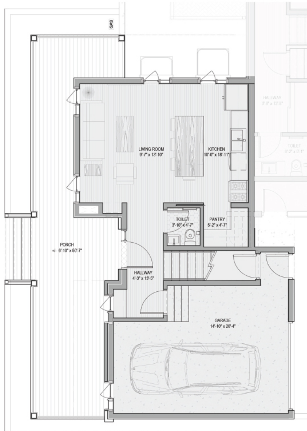
FIRST FLOOR
